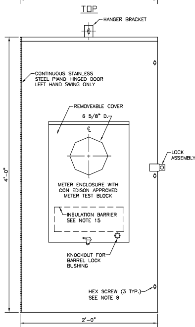
FRONT WITH METER COVER
