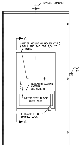
FRONT WITH METER COVER REMOVED SHOWING METER TEST BLOCK
