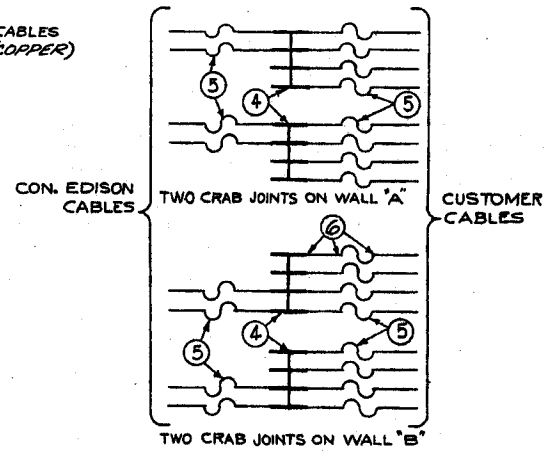
SCHEMATIC DIAGRAM OF CONNECTIONS FOR ONE PHASE
