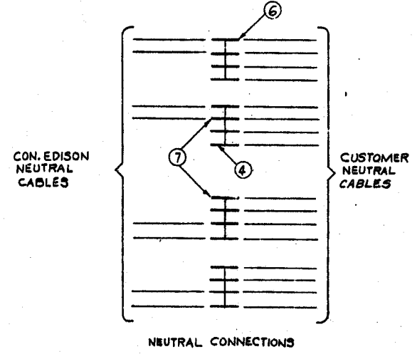
SCHEMATIC DIAGRAM OF CONNECTIONS FOR ONE PHASE
