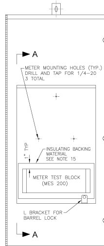
FRONT WITH METER COVER REMOVED SHOWING METER TEST BLOCK
