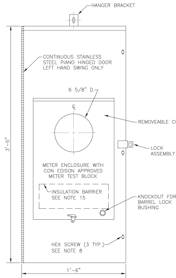
FRONT WITH METER COVER
