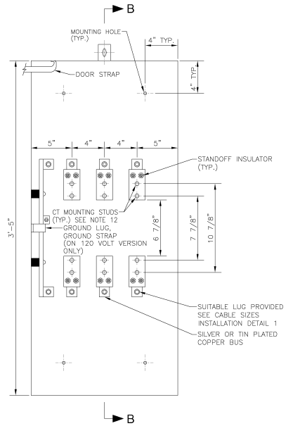
FRONT INSIDE VIEW
