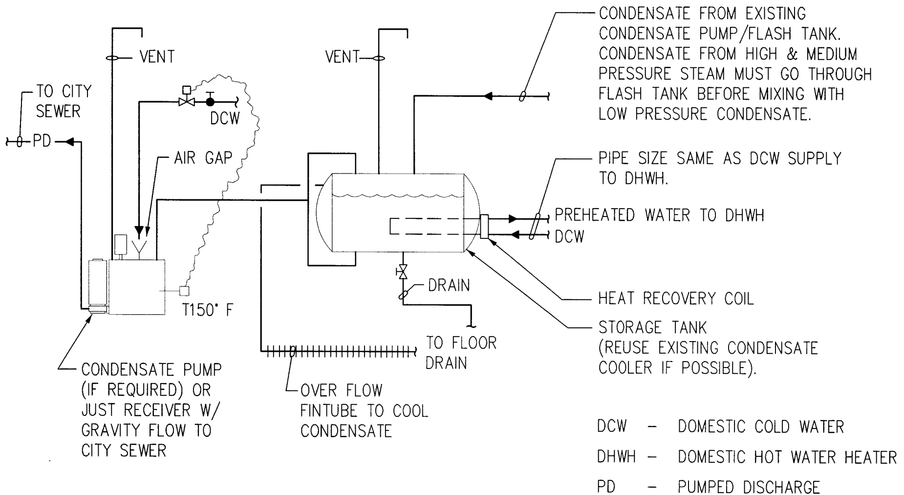
CONDENSATE REUSE TO PREHEAT DOMESTIC WATER GUIDANCE SKETCH - NOT TO SCALE
