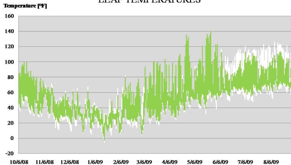
Figure 7: Comparative white and sedum plant leaf temperatures
